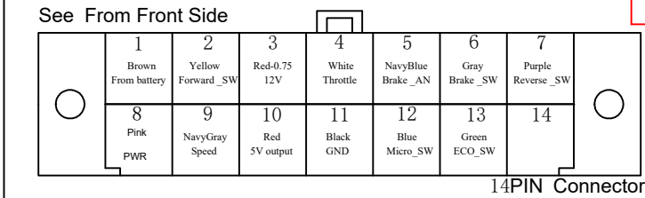
KLS-8080I/IPS 100G 120G Controller Assembly Wiring Diagram
