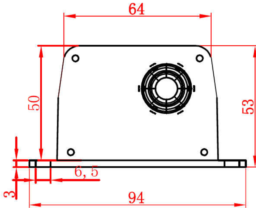
Fig.3 (Front view)
